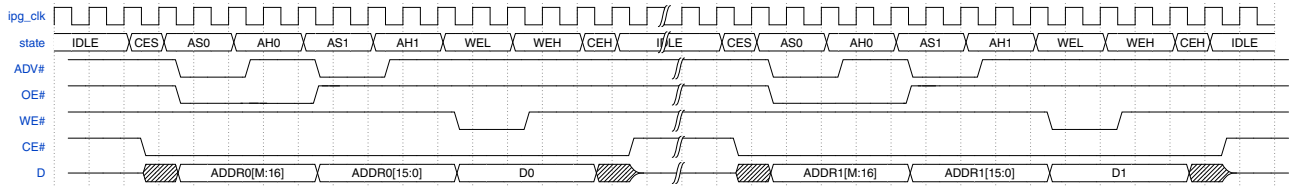
Figure 25-62. SRAM Write in ASYNC mode (AADM)
