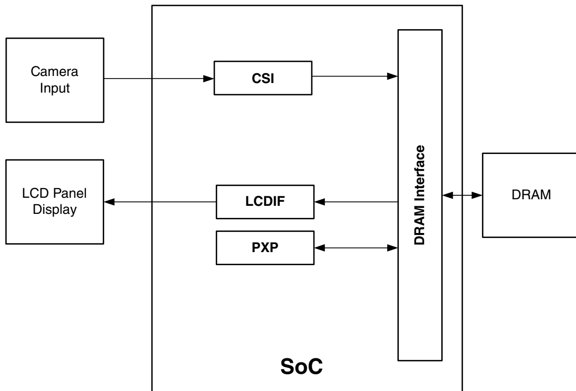
Figure 33-1. Block Diagram
