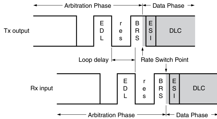
Figure 45-4. Transceiver loop delay measurement
