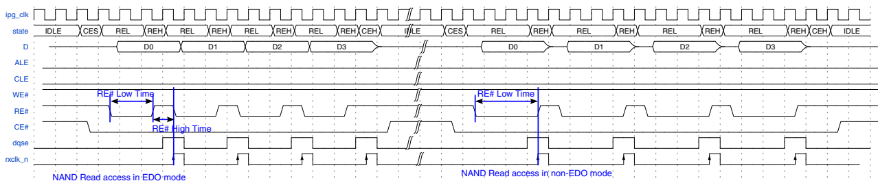
Figure 25-46. NAND Flash Read Access in EDO or non-EDO mode
