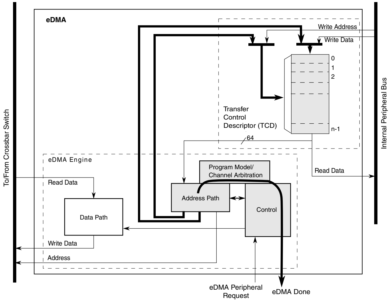
Figure 6-4. eDMA operation, part 3
