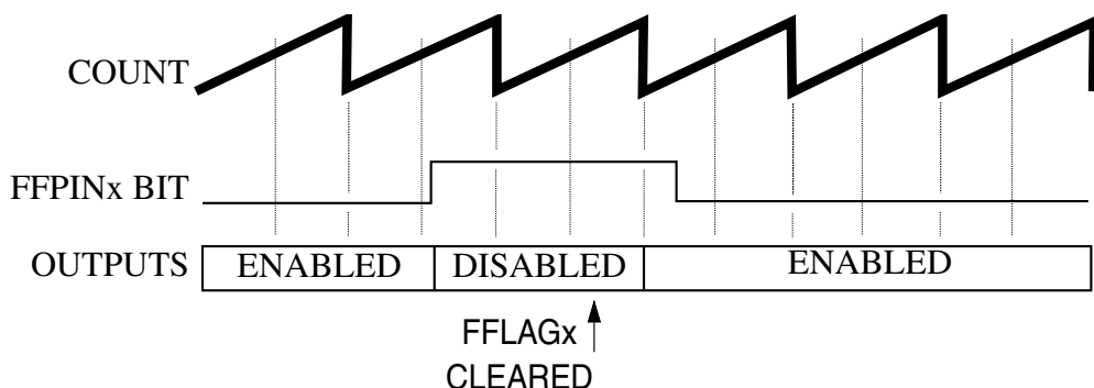
Figure 55-30. Manual Fault Clearing (FCTRL[FSAFE]=1)
