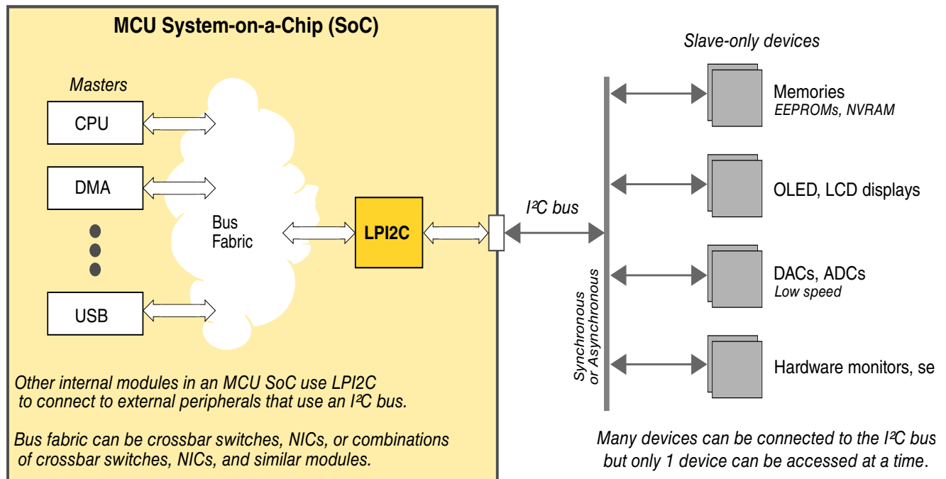
Figure 47-3. Typical LPI2C connection scheme
