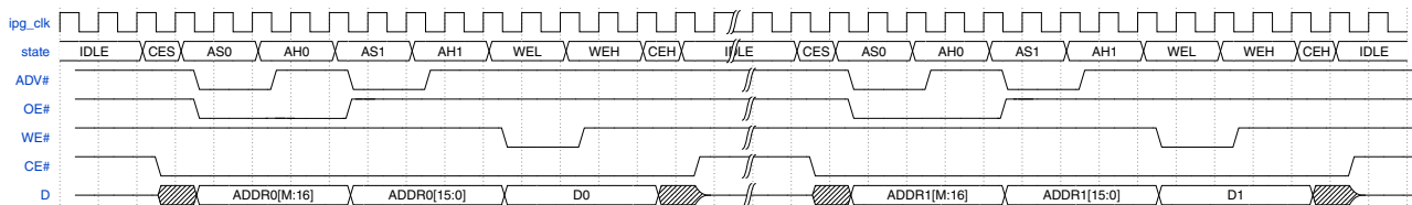
Figure 25-55. Flash Write in ASYNC mode (AADM)
