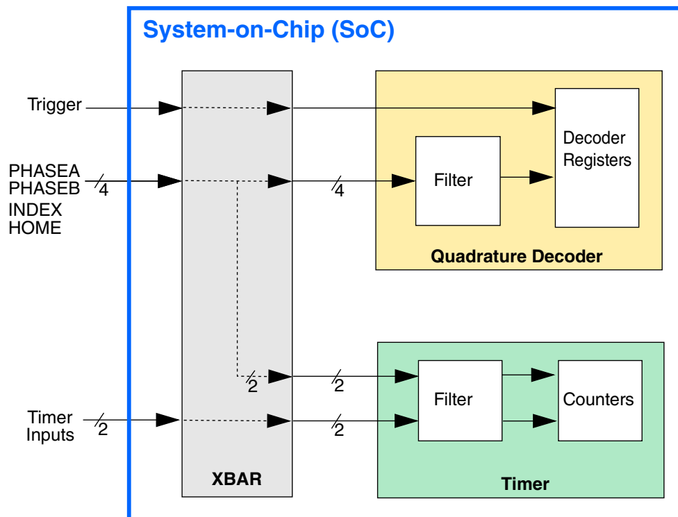
Figure 56-1. System Block Diagram
