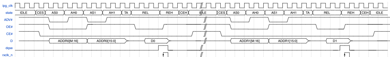
Figure 25-60. SRAM Read in ASYNC mode (AADM)
