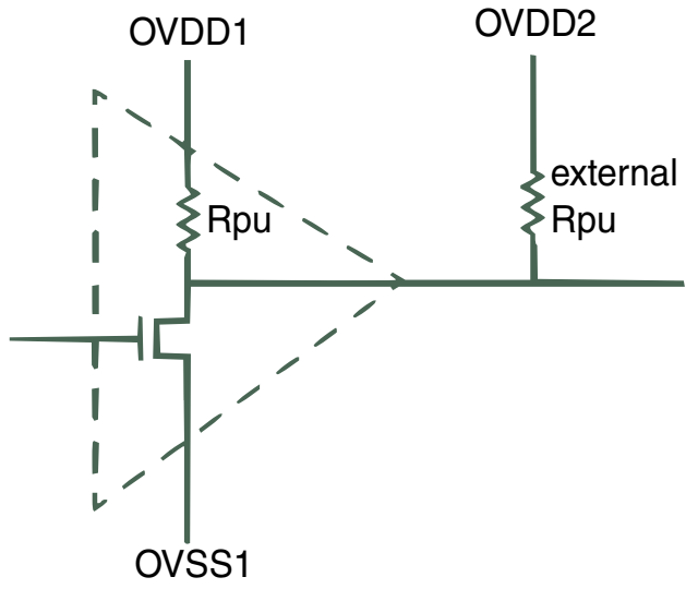
Figure 12-8. Output buffer in open drain mode
