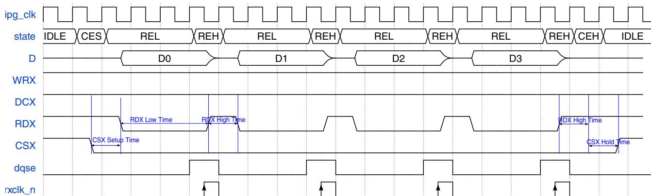
Figure 25-66. DBI Read Operation
