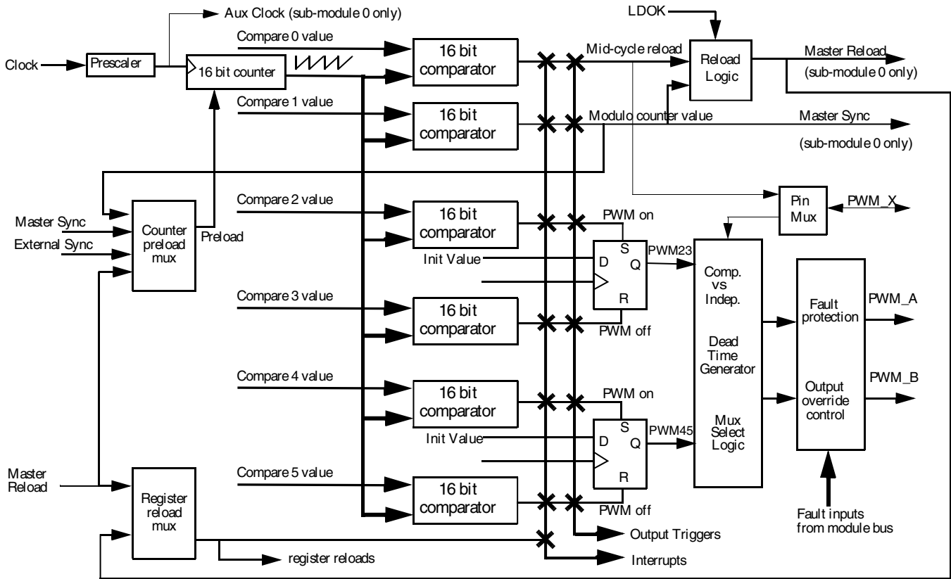
Figure 55-1. PWM Submodule Block Diagram
