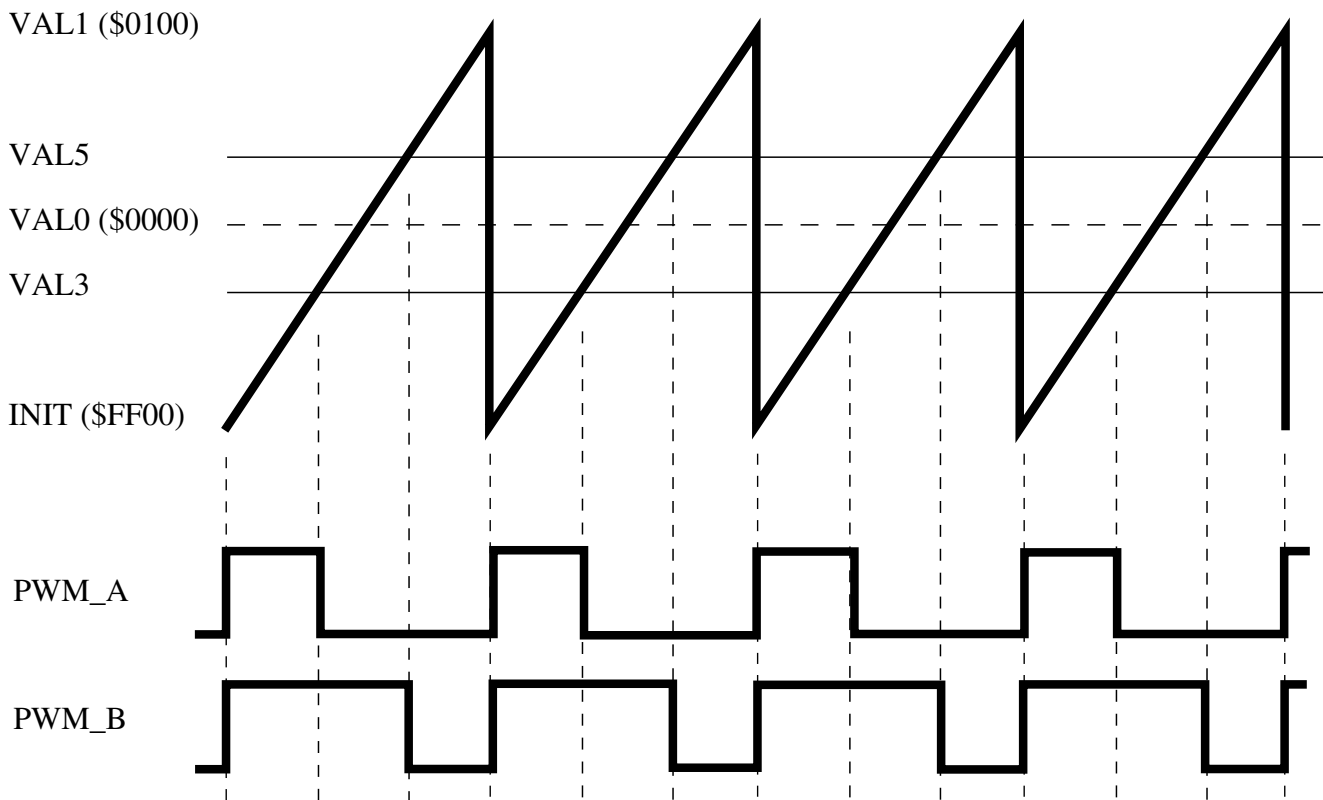
Figure 55-3. Edge Aligned Example (INIT=VAL2=VAL4)
