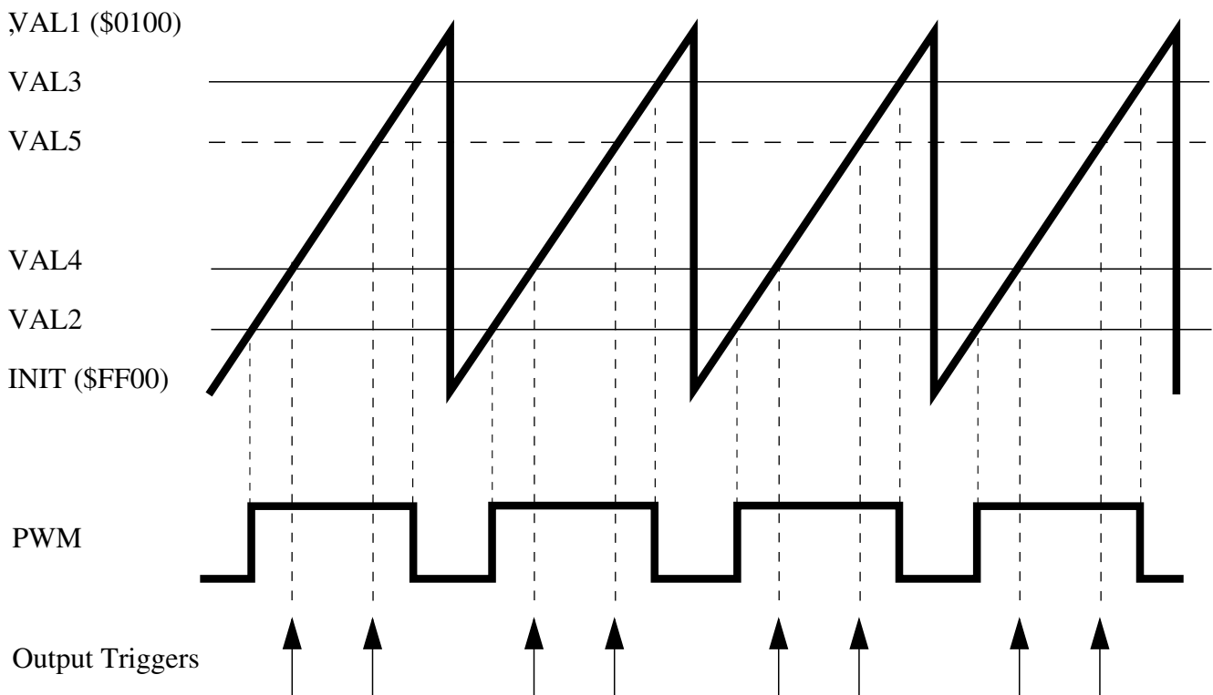
Figure 55-7. Multiple Output Trigger Generation in Hardware
