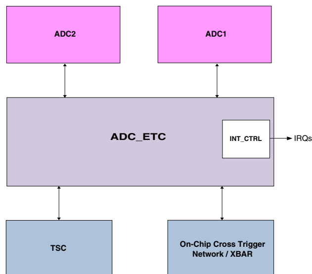
Figure 64-1. Block Diagram (Simplified)
