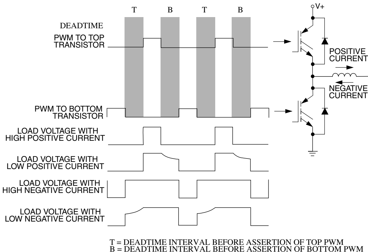
Figure 55-24. Output Voltage Waveforms
