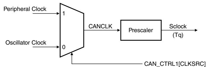
Figure 45-6. CAN engine clocking scheme
