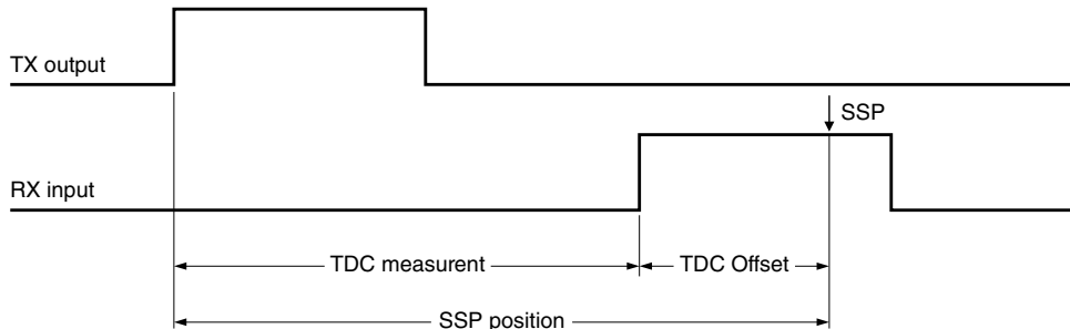
Figure 45-5. SSP position with optimal values
