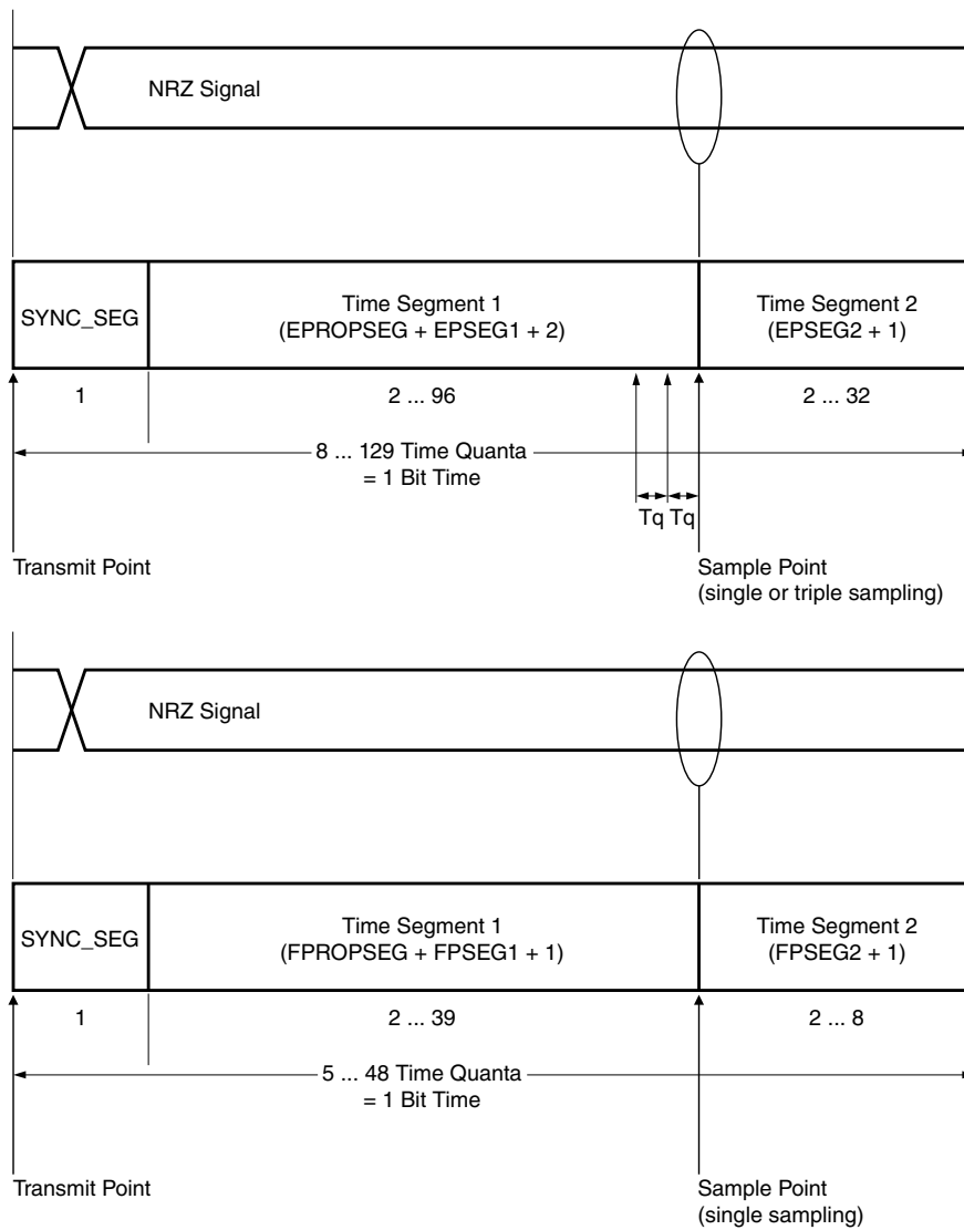
Figure 45-8. Segments within the bit time (example using CBT and FDCBT bit timing variables for CAN FD format)
