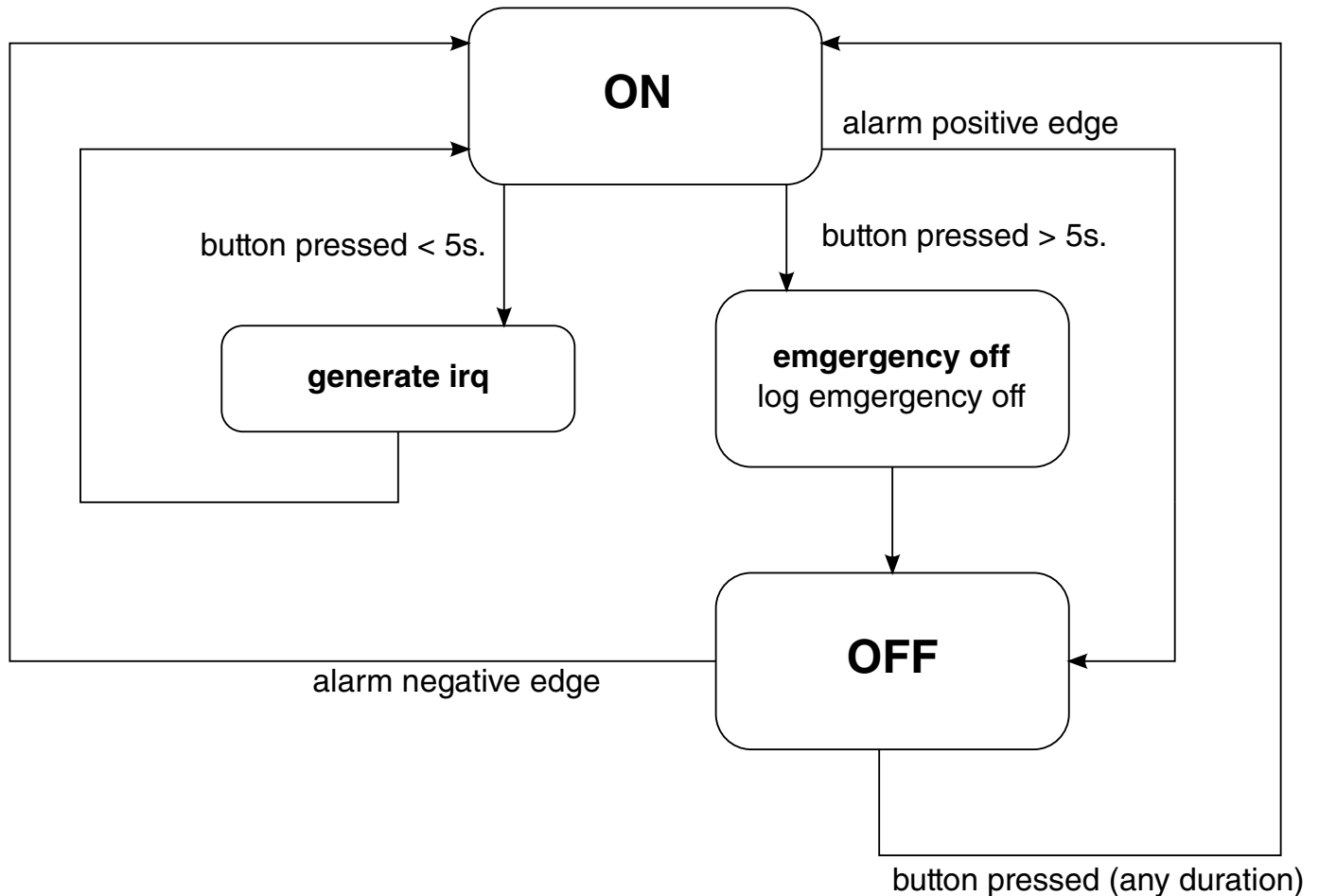
Figure 21-4. FSM
