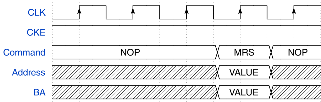
Figure 25-5. IP command - SDRAM MODE REGISTER SET
