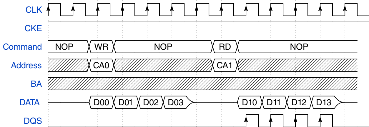
Figure 25-22. SDRAM Write-to-Read access (CL=1)
