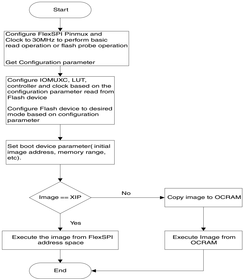
Figure 9-3. FlexSPI NOR boot flow
