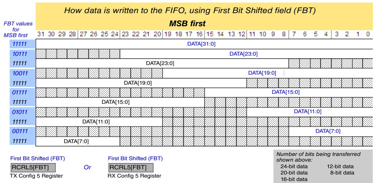
Figure 38-3. SAI first bit shifted, MSB first
