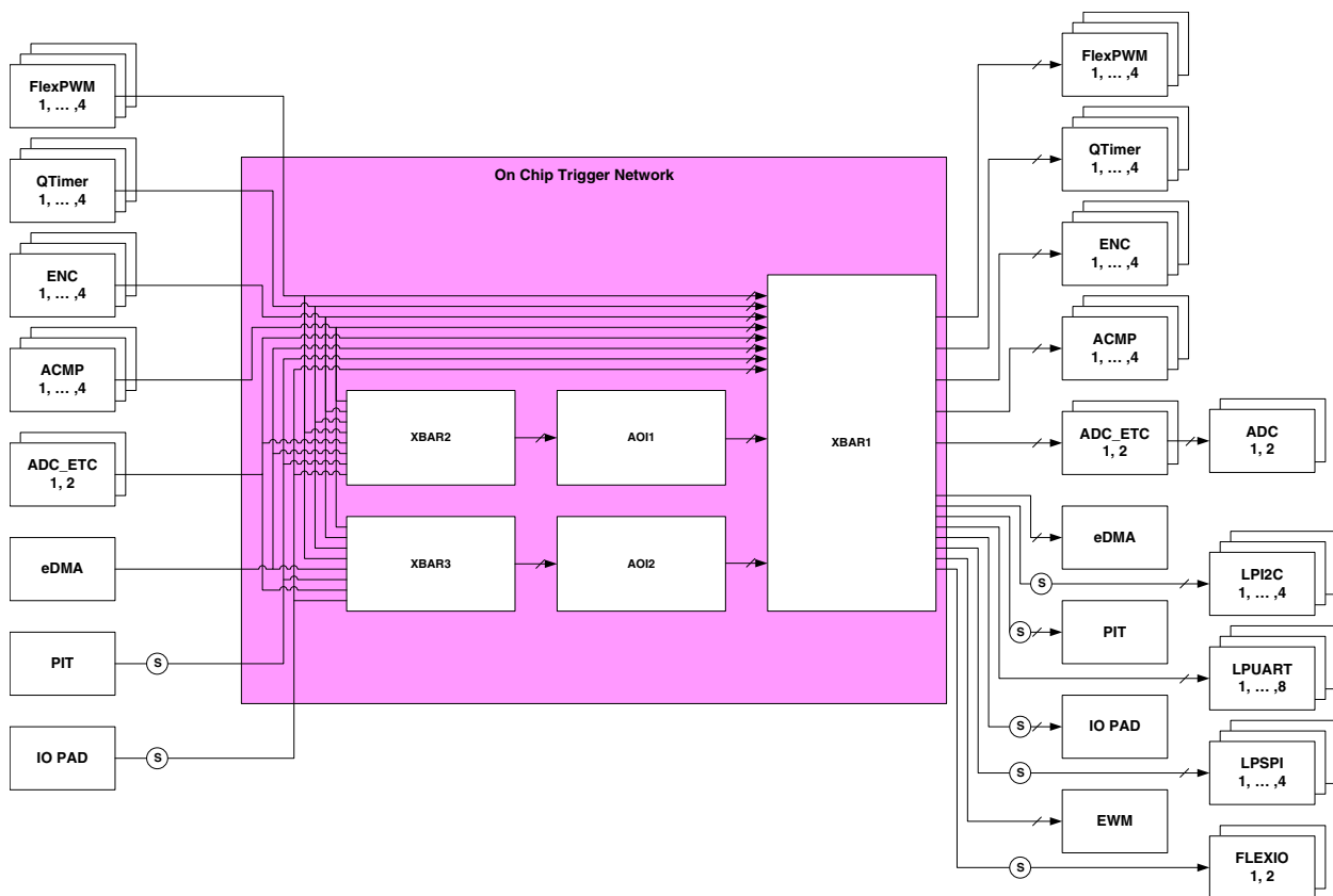
Figure 60-1. On-Chip Cross Trigger Network
