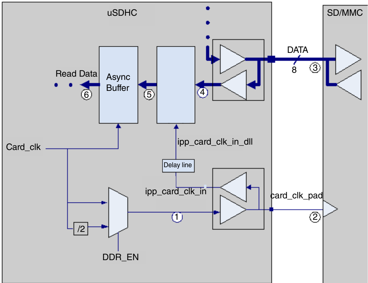
Figure 26-20. DLL(Delay Line) in Read Path
