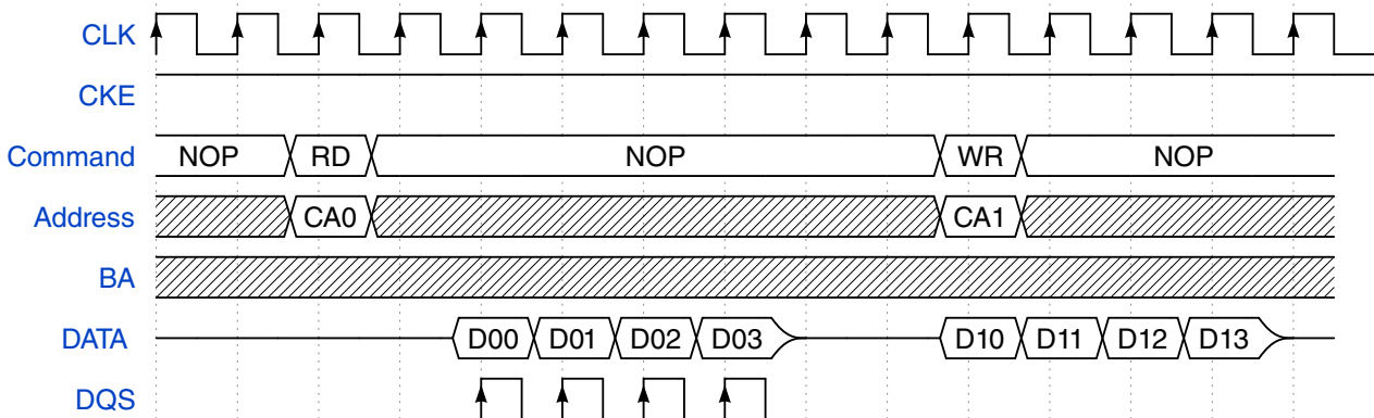
Figure 25-19. SDRAM Read-to-Write access (CL=2)
