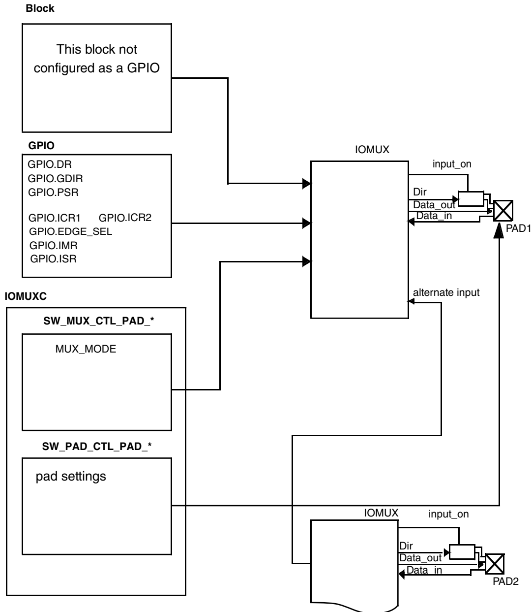
Figure 12-1. Chip IOMUX Scheme
