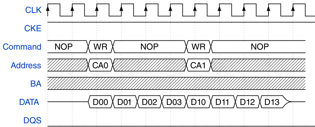
Figure 25-21. SDRAM Write-to-Write access
