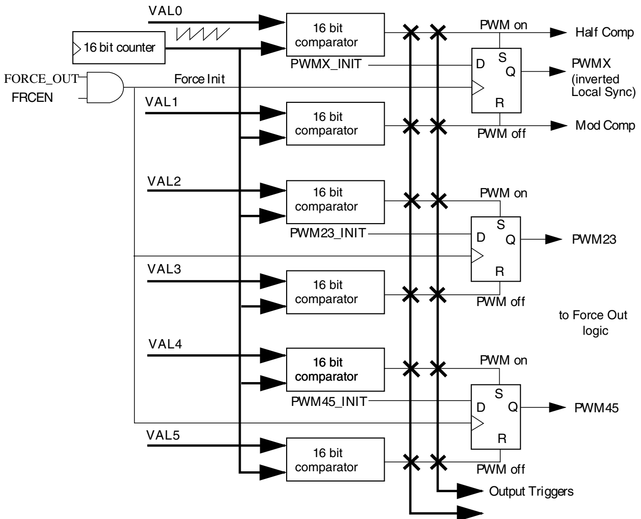
Figure 55-16. PWM Generation Hardware
