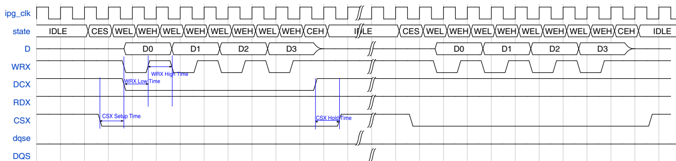
Figure 25-65. DBI Write Operation
