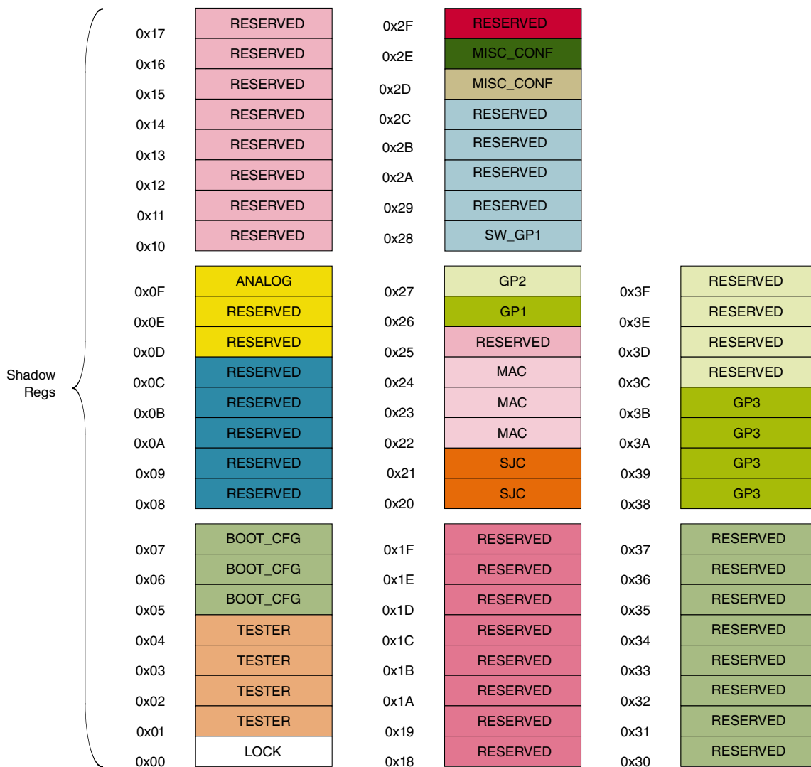
Figure 23-2. OTP Memory Footprint
