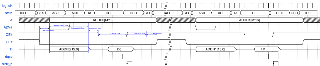
Figure 25-59. SRAM Read in ASYNC mode (ADMUX)
