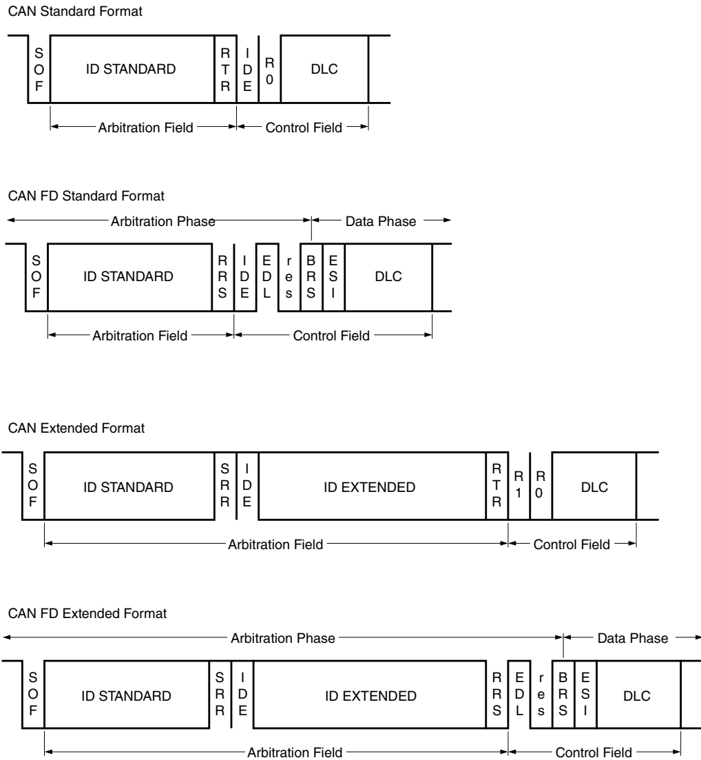
Figure 45-2. CAN message formats
