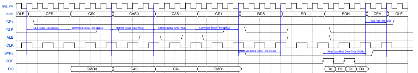
Figure 25-49. NAND Command + Address + Command + Read in SYNC mode
