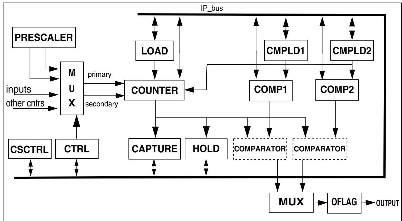
Figure 54-1. Quad Timer Block Diagram
