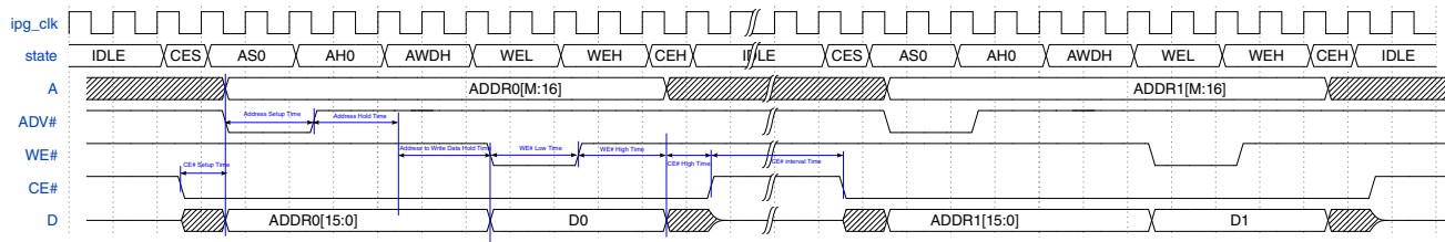
Figure 25-54. Flash Write in ASYNC mode (ADMUX)
