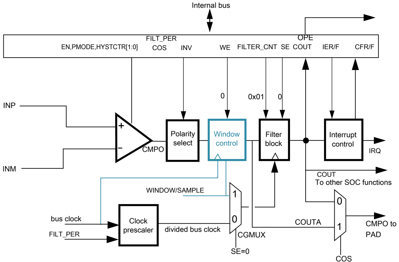
Figure 65-5. Sampled, Non-Filtered (# 3B): sampling interval internally derived
