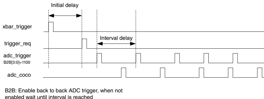
Figure 67-3. ETC ADC interface timing
