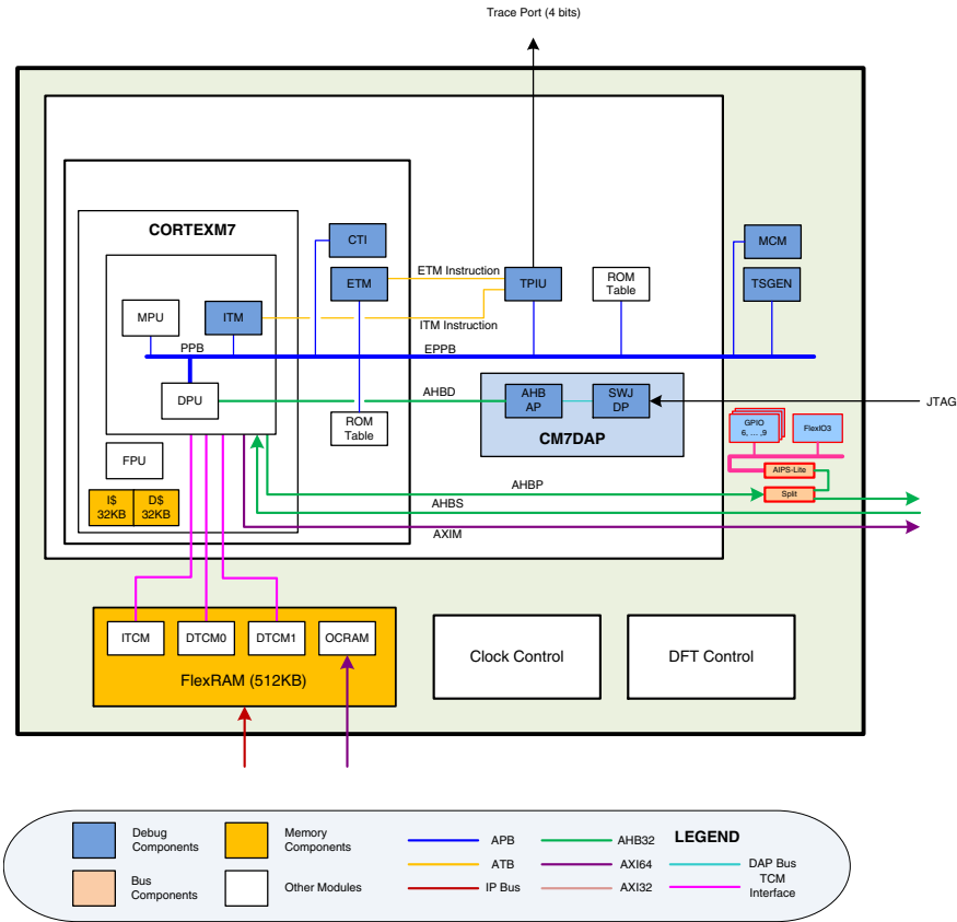
Figure 28-1. Cortex-M7 Platform Block Diagram
