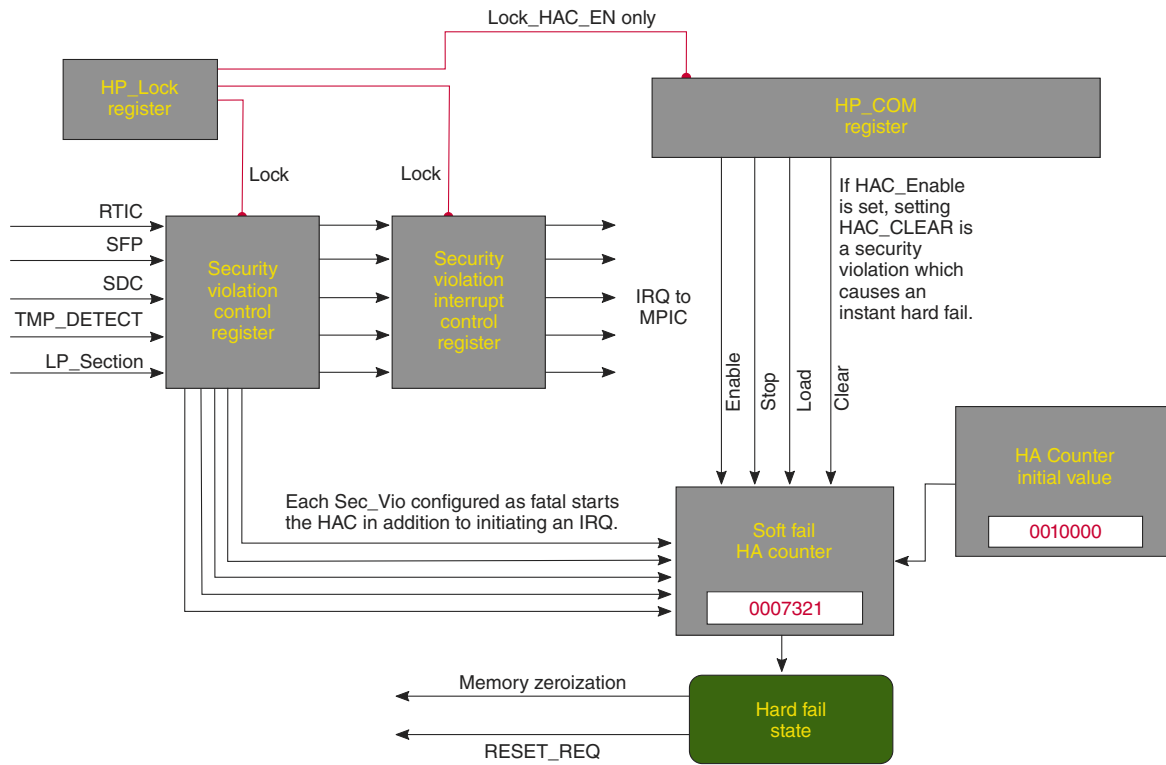
Figure 20-1. Relationship Between the Registers
