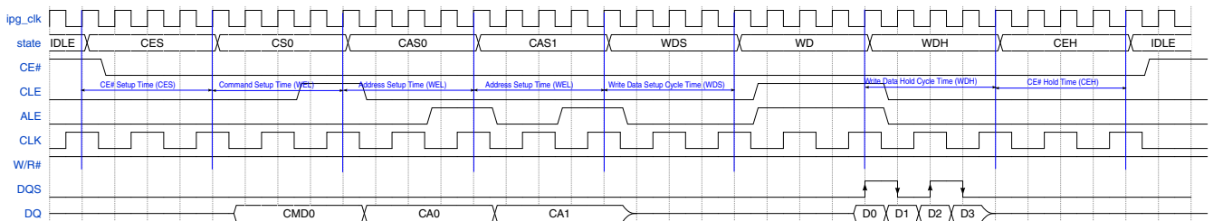
Figure 25-50. NAND Command + Address + Write in SYNC mode
