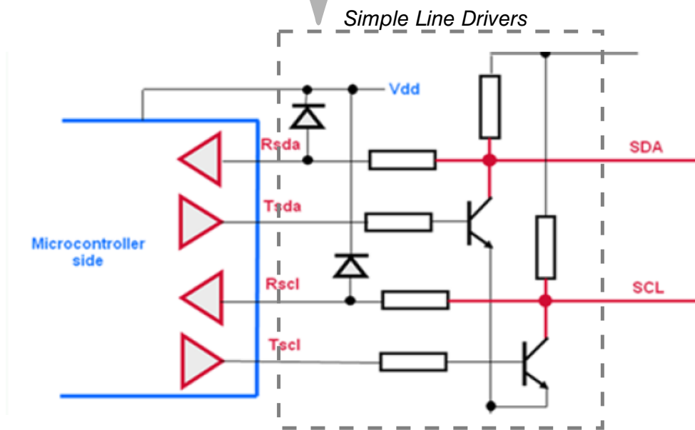
Figure 47-6. 4-Wire scheme
