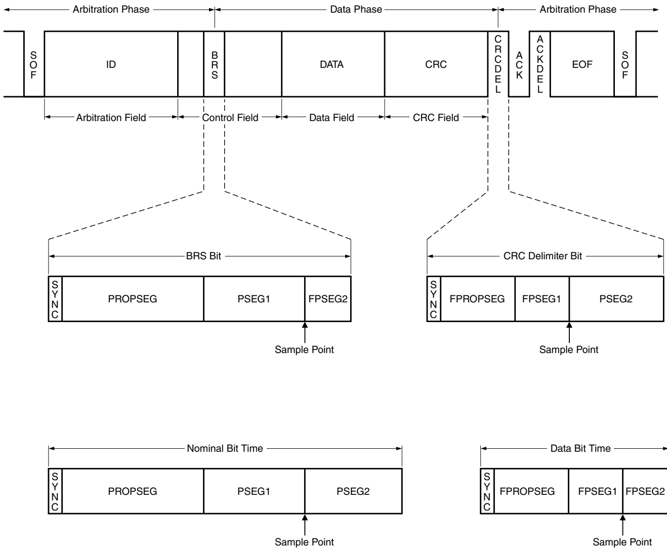
Figure 45-3. Bit rate switching mechanism for CAN FD messages
