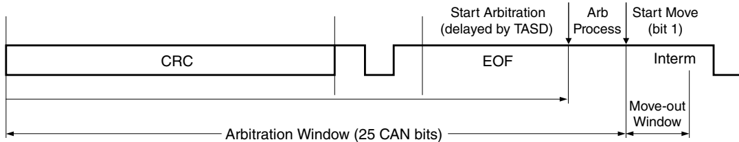
Figure 45-10. Arbitration and move-out time windows
