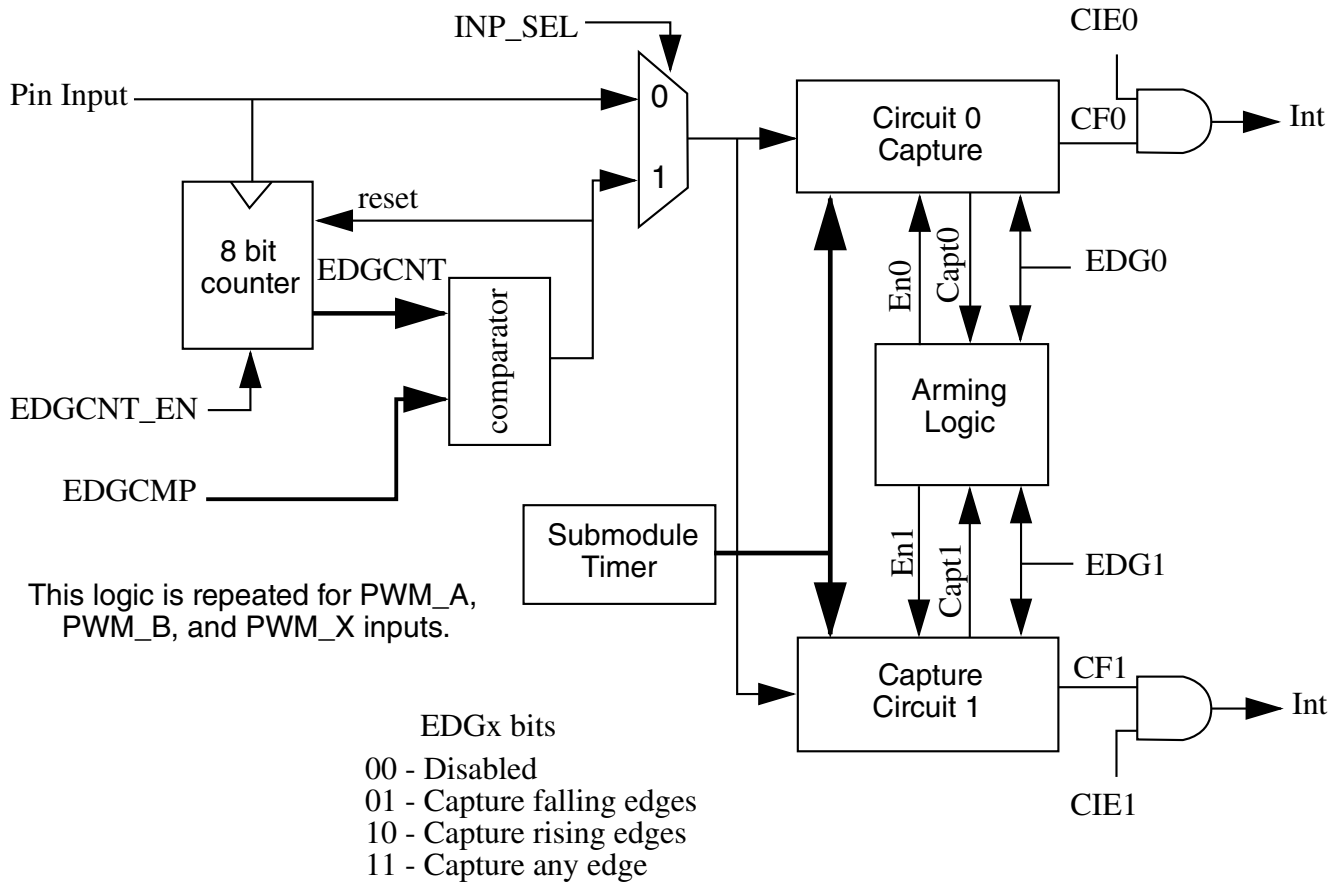
Figure 55-26. Enhanced Capture (E-Capture) Logic
