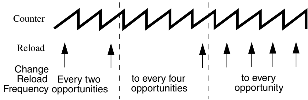
Figure 55-32. Half Cycle Reload Frequency Change
