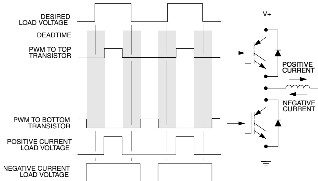
Figure 55-22. Deadtime Distortion
