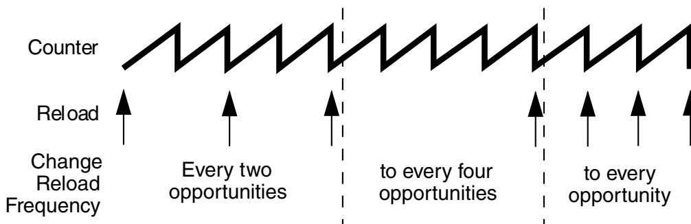
Figure 55-31. Full Cycle Reload Frequency Change
