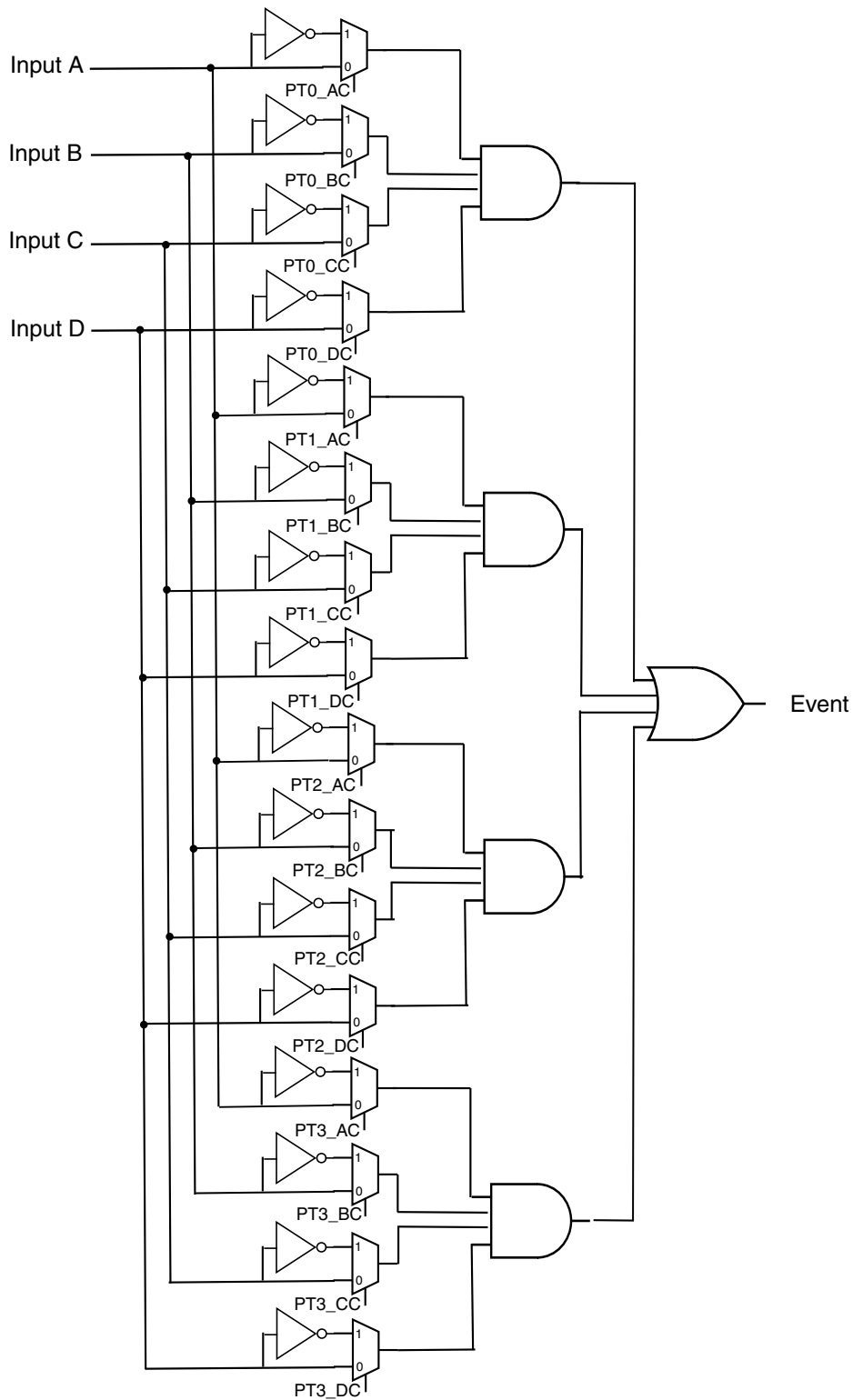
Figure 63-1. Simplified AOI Block Diagram
