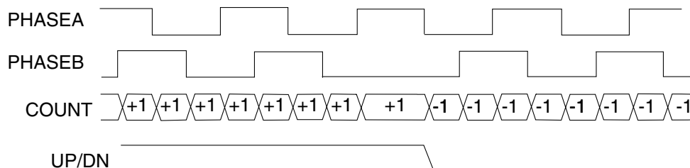
Figure 54-3. Quadrature Incremental Position Encoder
