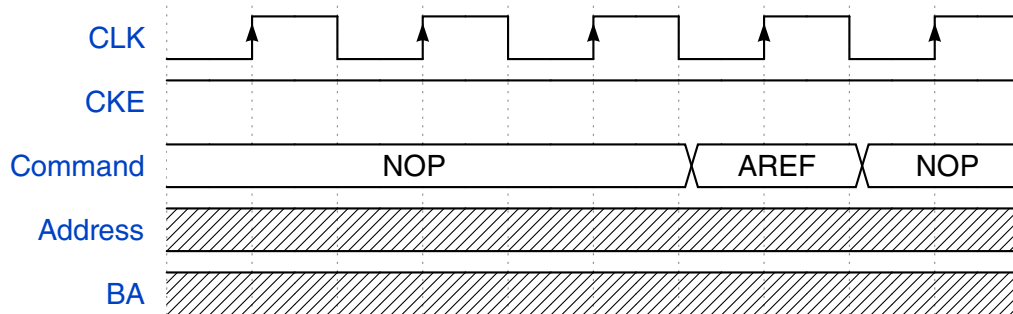
Figure 25-4. IP command - SDRAM Auto Refresh
