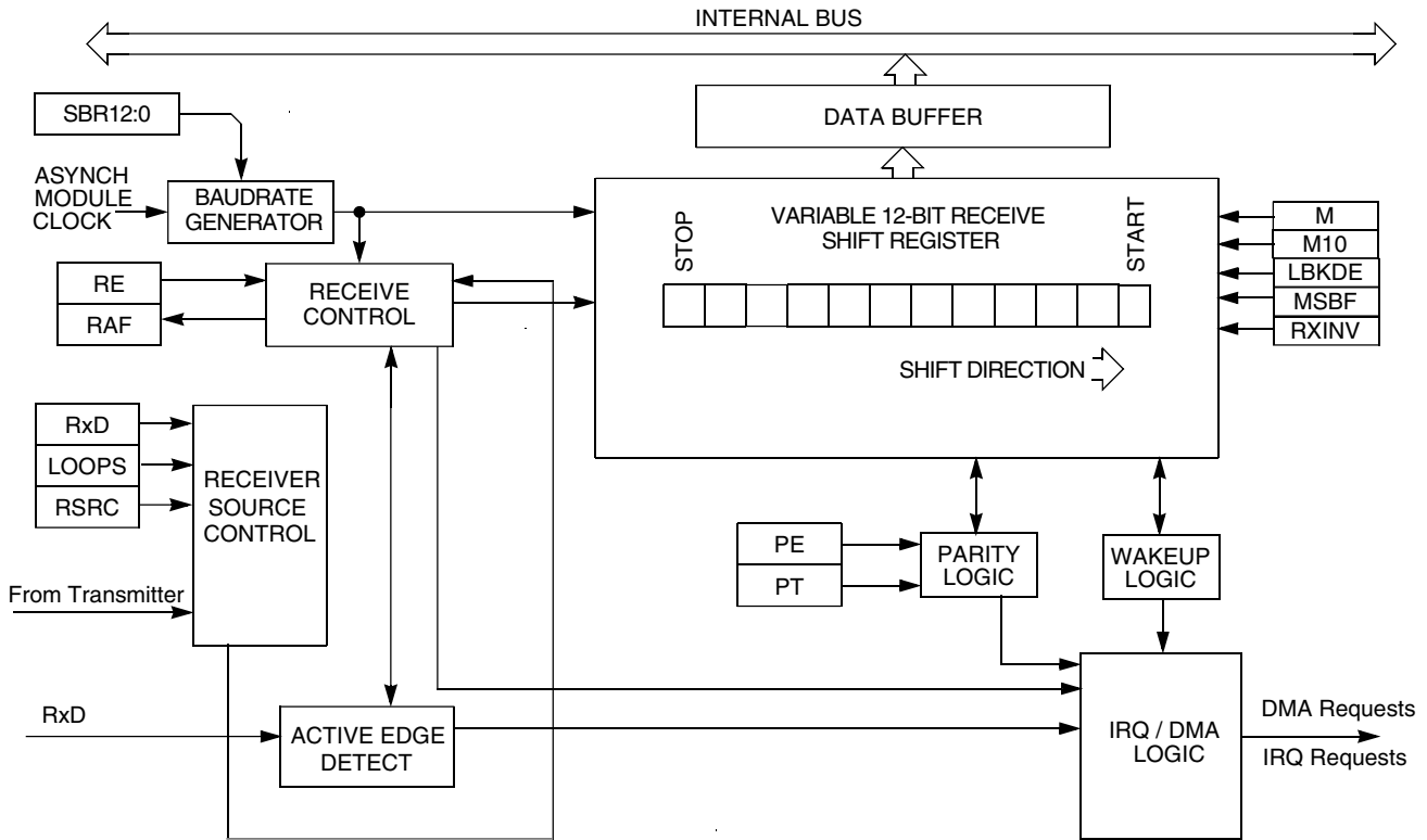
Figure 49-2. LPUART receiver block diagram
