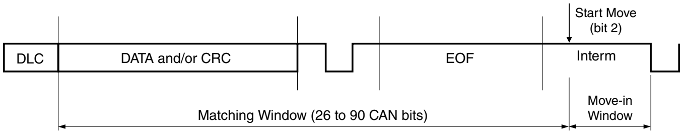
Figure 45-9. Matching and move-in time windows
