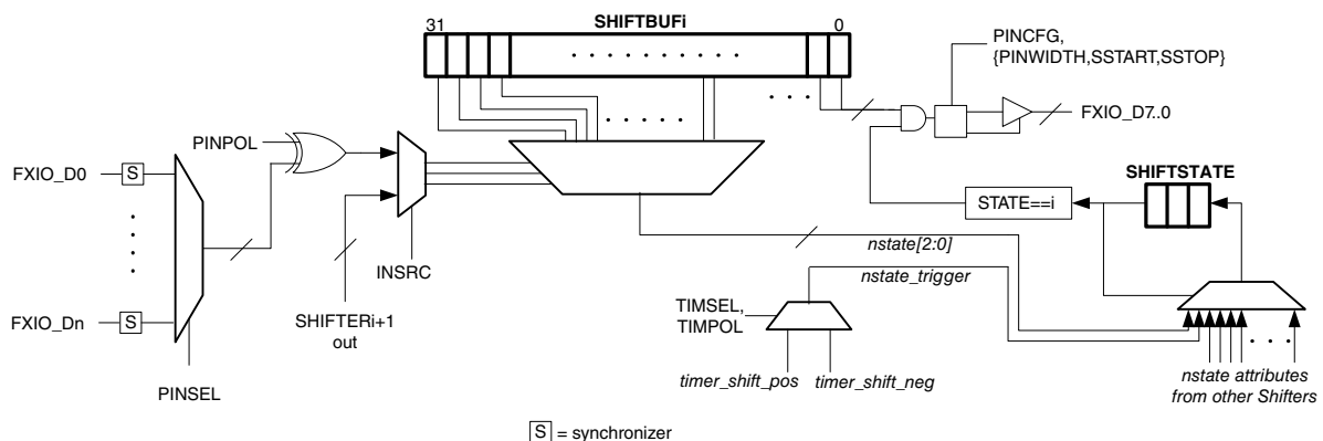
Figure 50-3. State Microarchitecture
