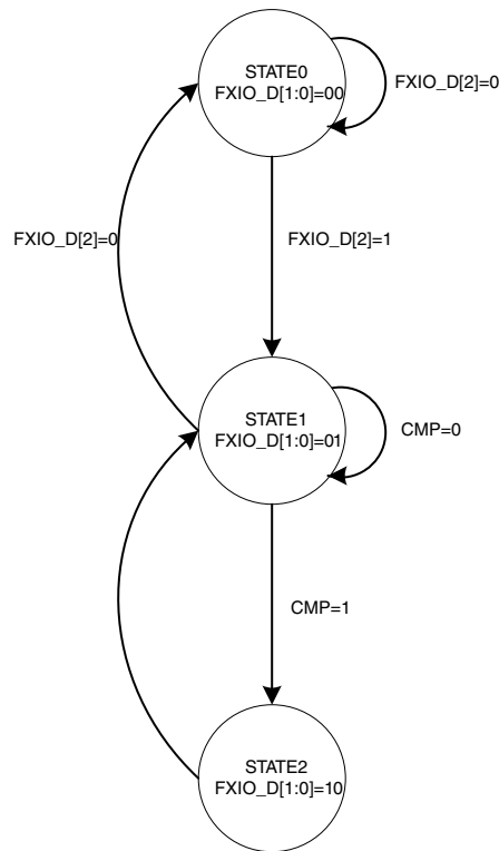
Figure 50-5. State Diagram
