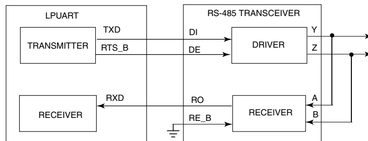
Figure 49-4. Transceiver driver enable using RTS_B
