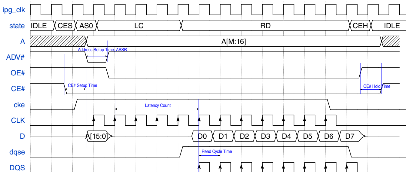
Figure 25-56. Flash Read in SYNC mode (ADMUX)
