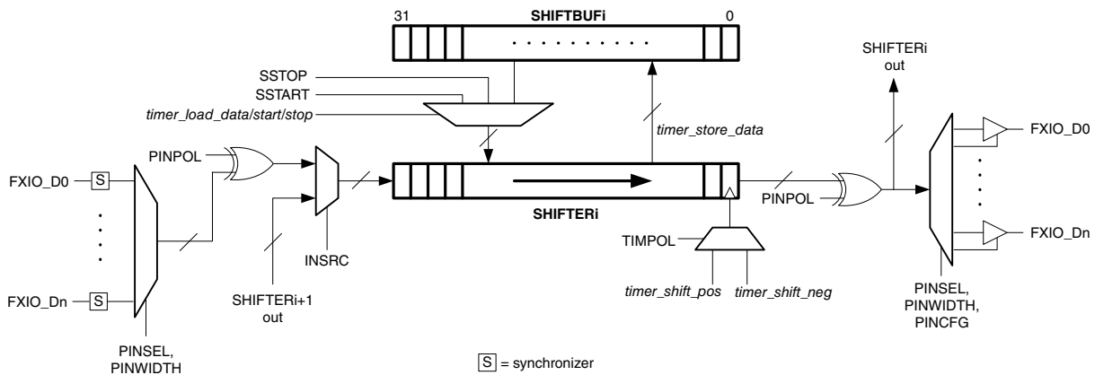
Figure 50-2. Shifter Microarchitecture
