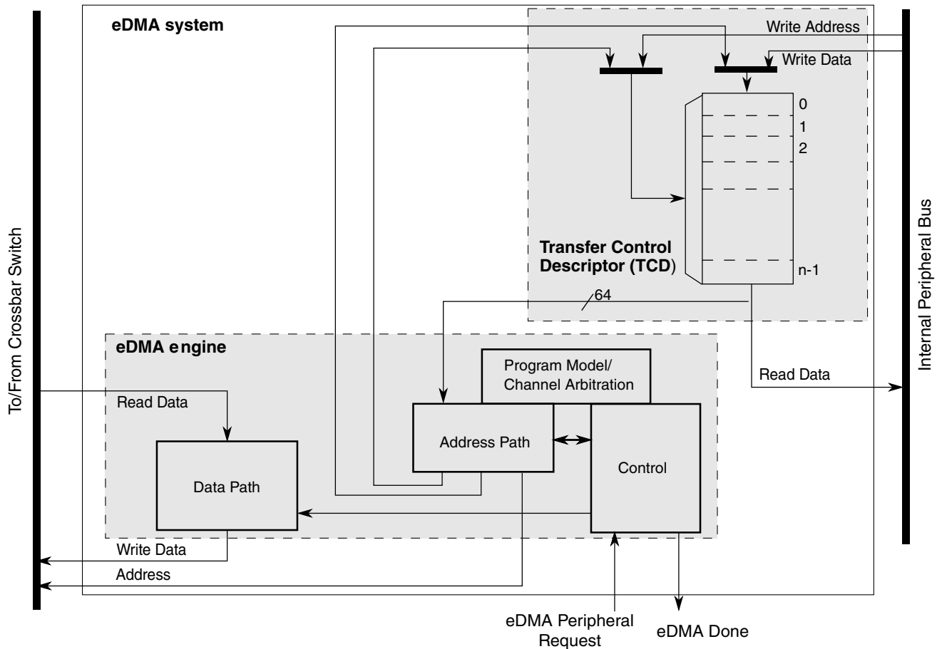
Figure 6-1. eDMA system block diagram
