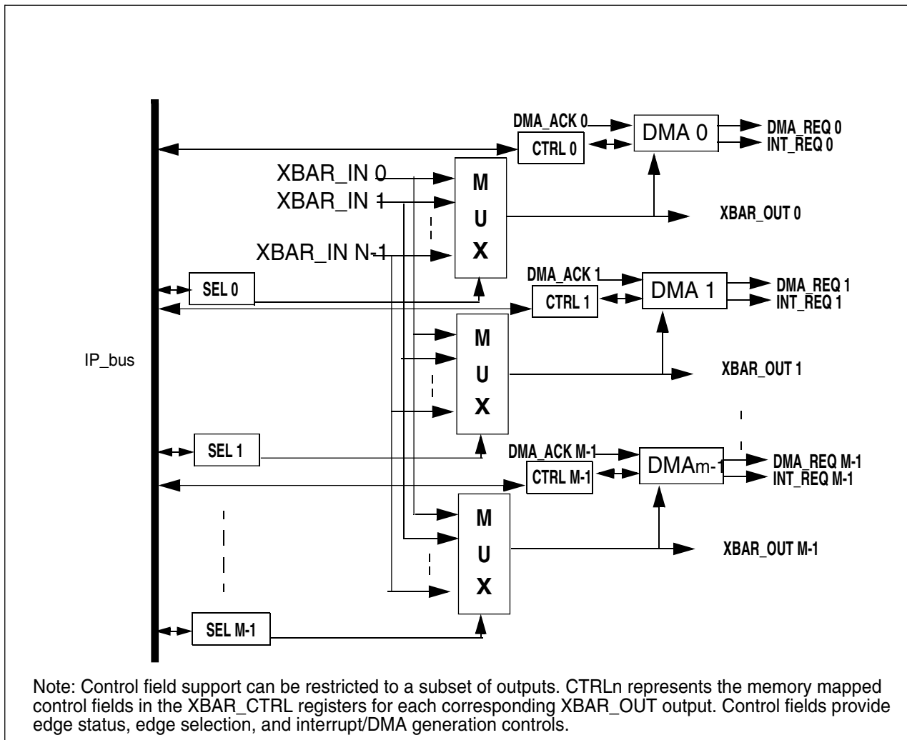
Figure 61-1. XBAR Block Diagram
