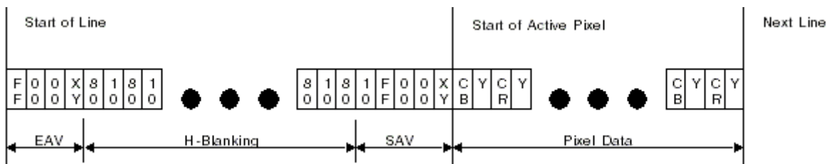
Figure 34-3. CCIR656 General Line Timing
