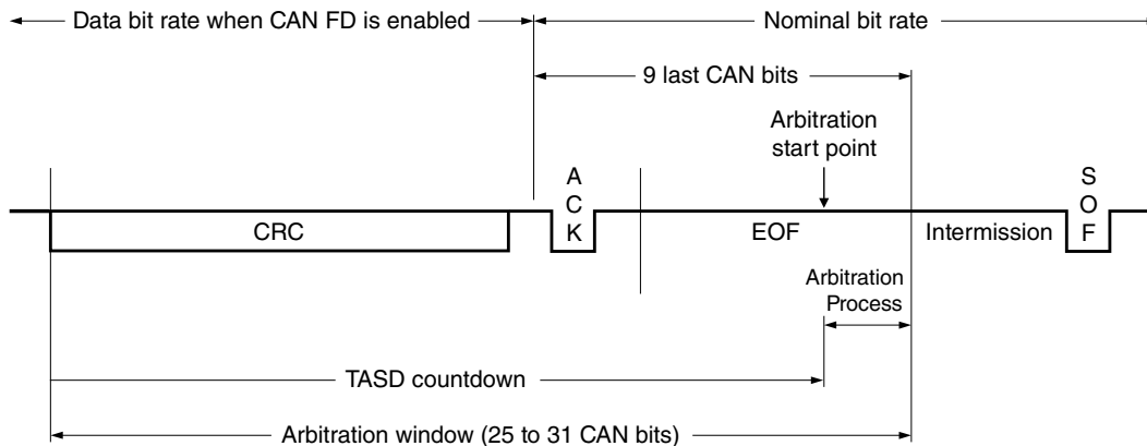
Figure 45-12. Optimal Tx Arbitration start point
