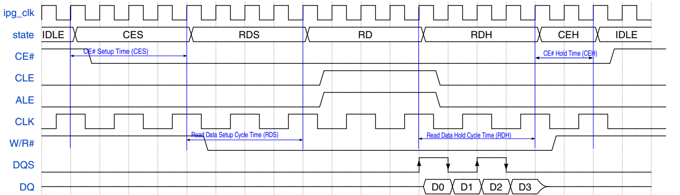
Figure 25-47. NAND Read in SYNC mode
