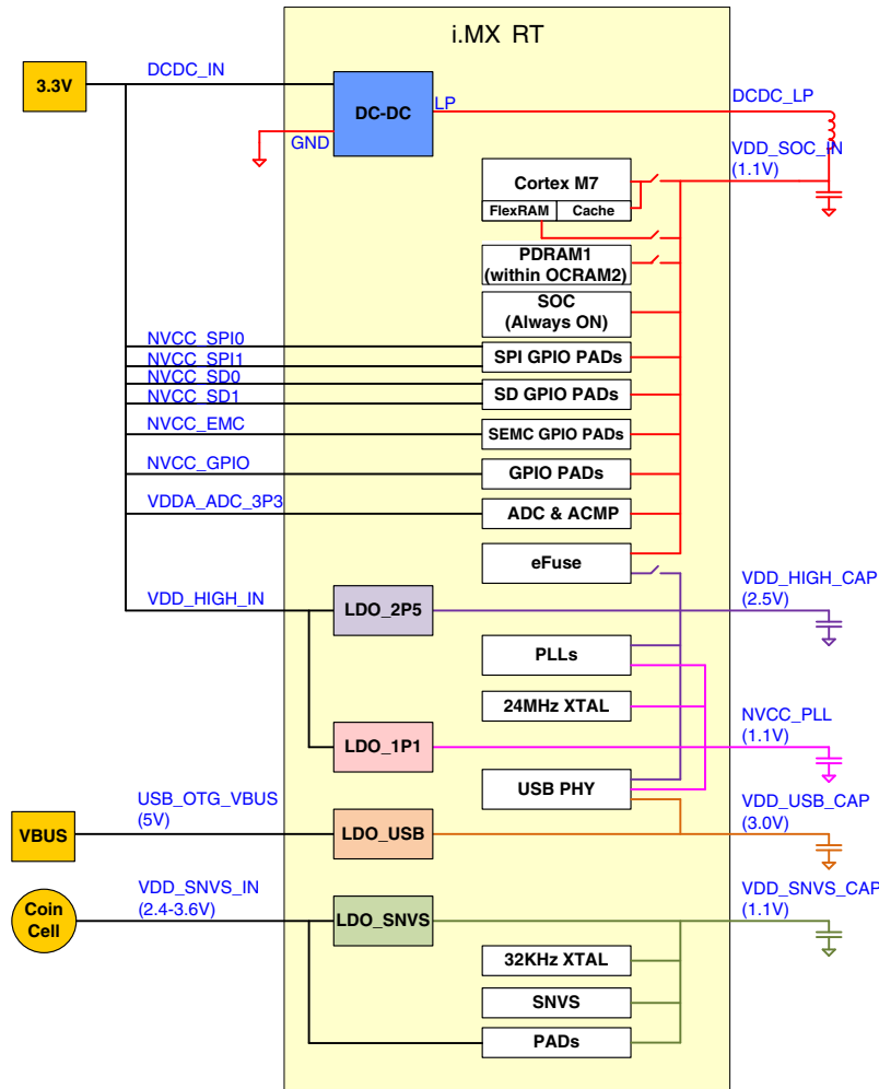
Figure 13-8. SOC Power Architecture
