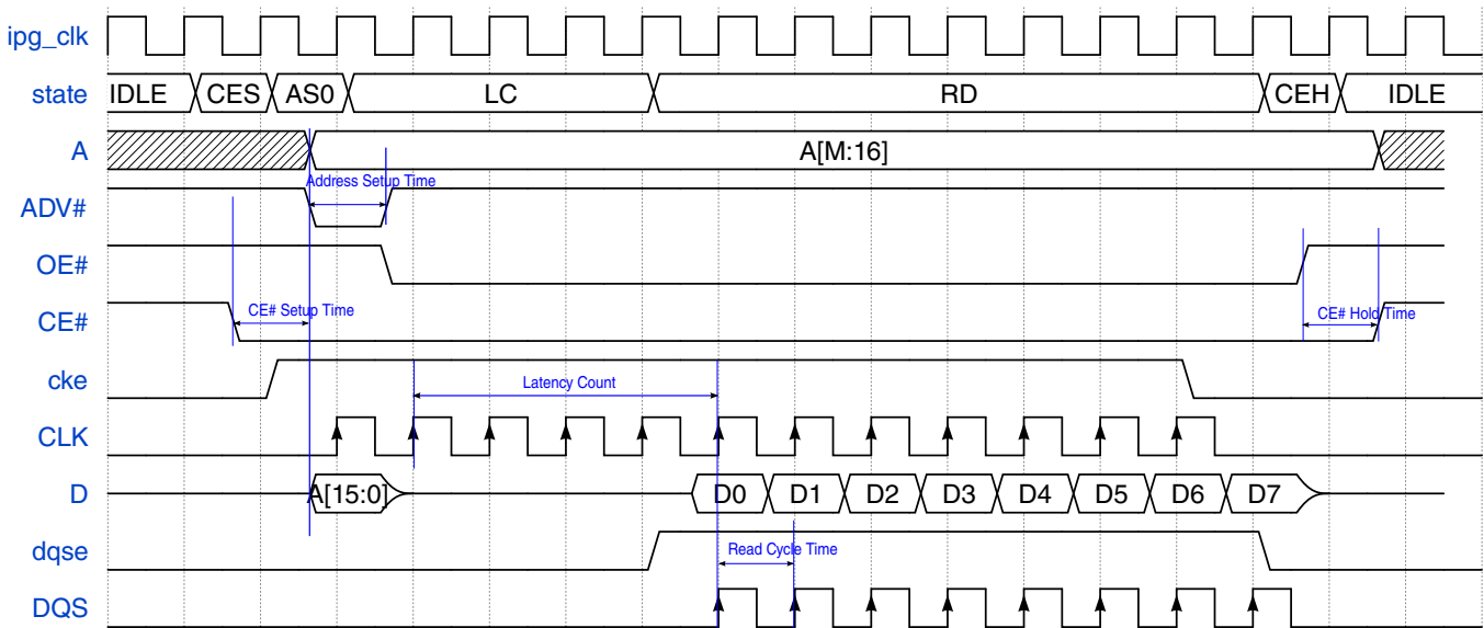
Figure 25-63. SRAM Read in SYNC mode (ADMUX)
