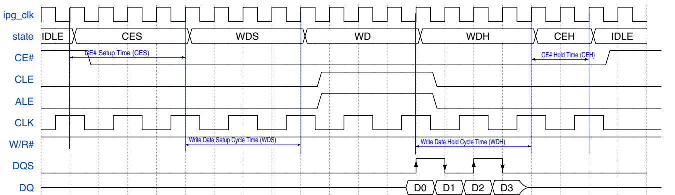
Figure 25-48. NAND Write in SYNC mode
