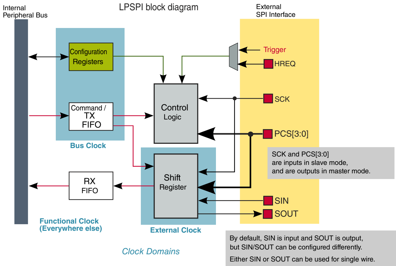
Figure 48-1. Block Diagram
