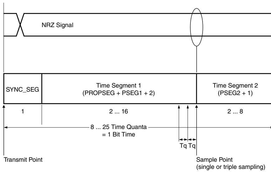
Figure 45-7. Segments within the bit time (example using CTRL1 bit timing variables for Classical CAN format)
