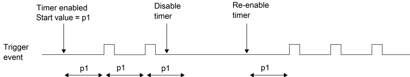
Figure 53-2. Stopping and starting a timer
