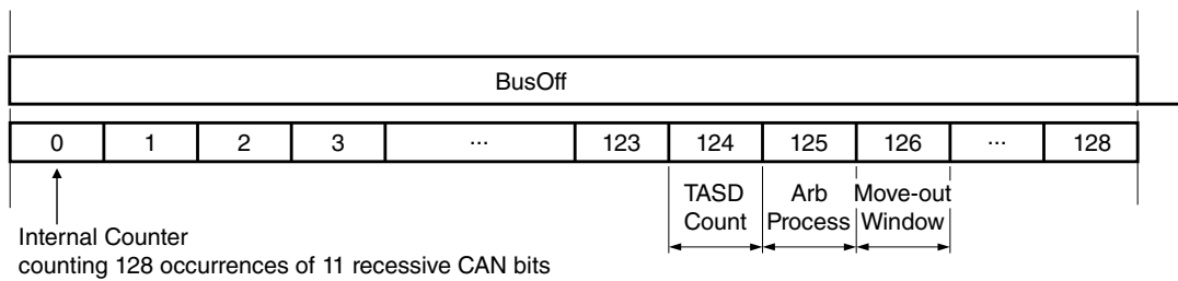
Figure 45-11. Arbitration at the end of bus off and move-out time windows
