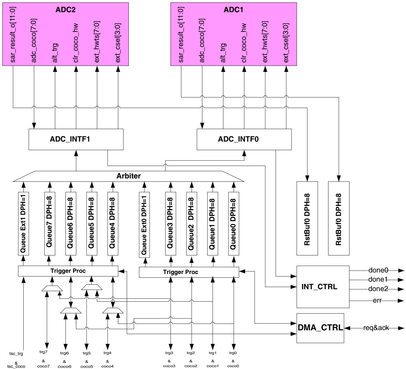
Figure 67-1. ADC_ETC block diagram
