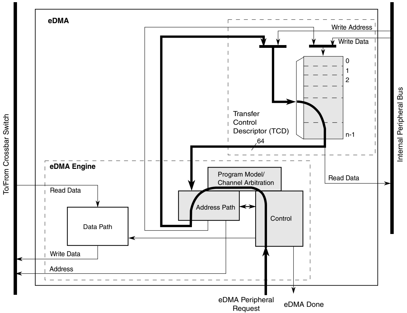
Figure 6-2. eDMA operation, part 1
