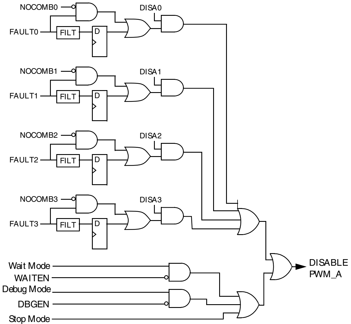
Figure 55-27. Fault Decoder for PWM_A
