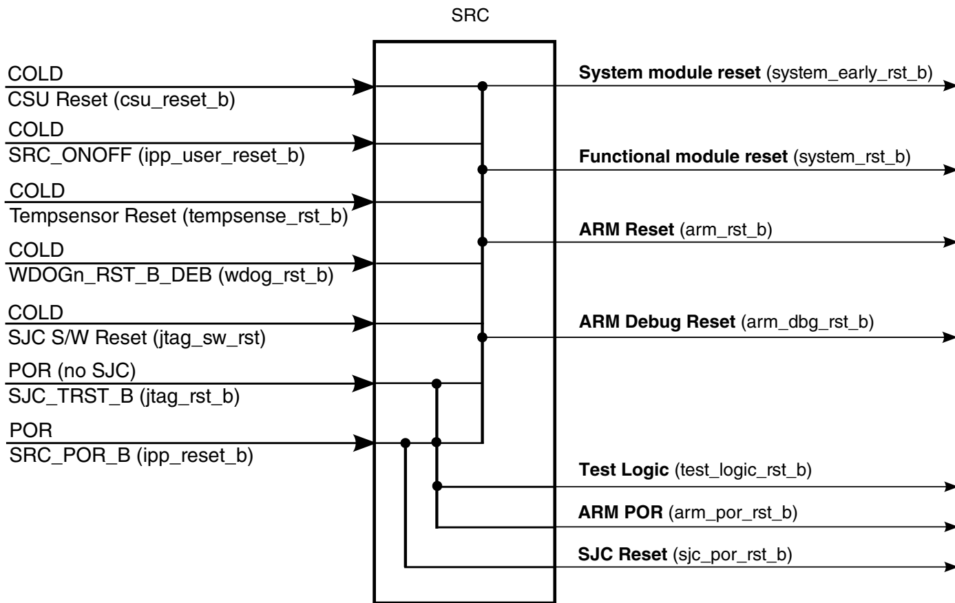
Figure 21-5. SRC inputs and outputs
