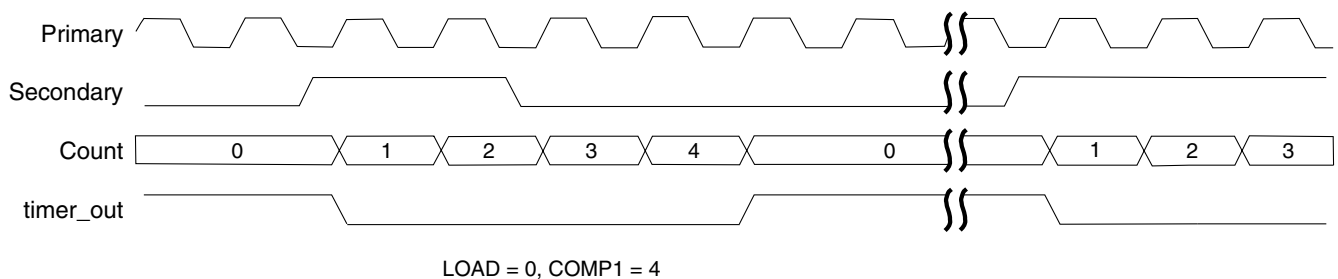
Figure 54-6. One-Shot Mode (CTRL[LENGTH]=1)
