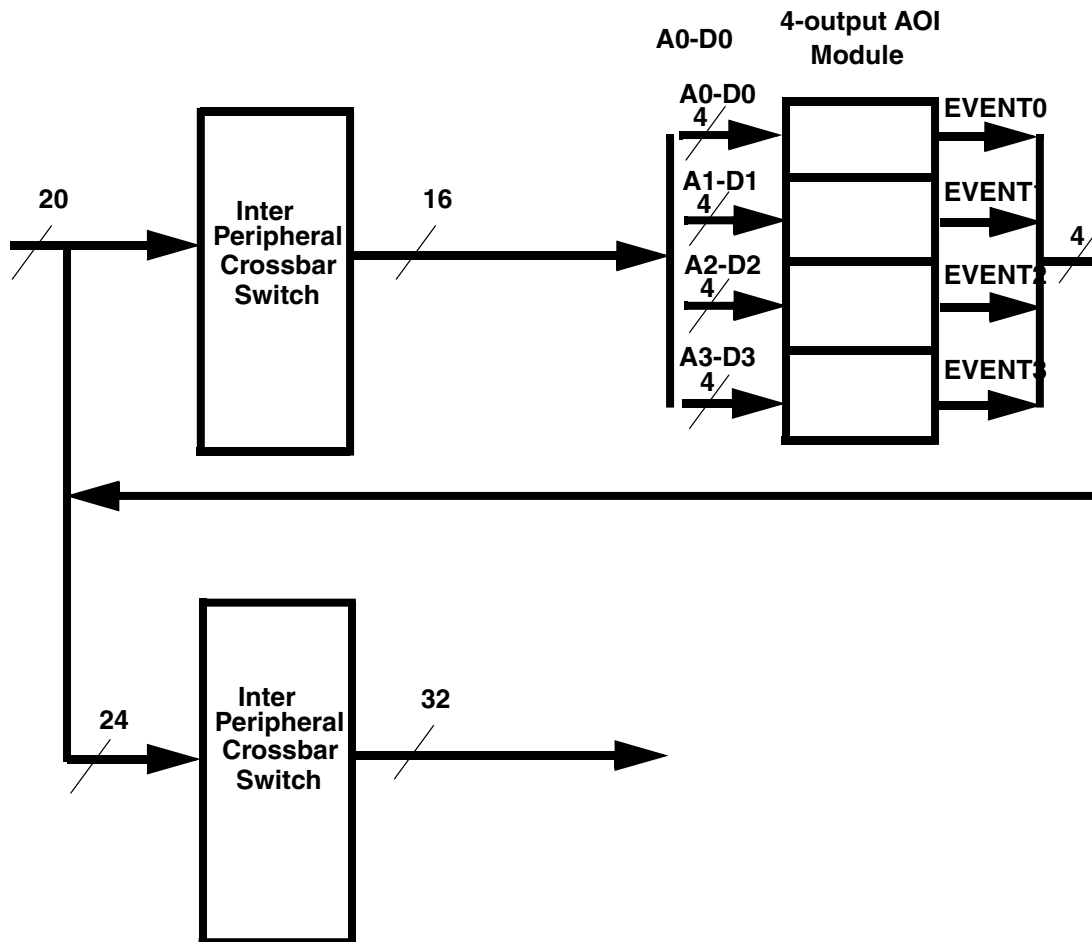
Figure 63-2. Integration Example of AOI with two Inter-Peripheral Crossbar Switches
