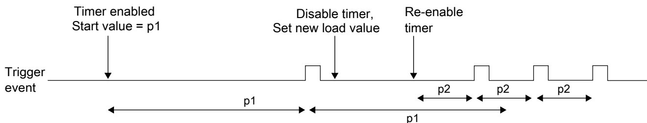
Figure 53-3. Modifying running timer period
