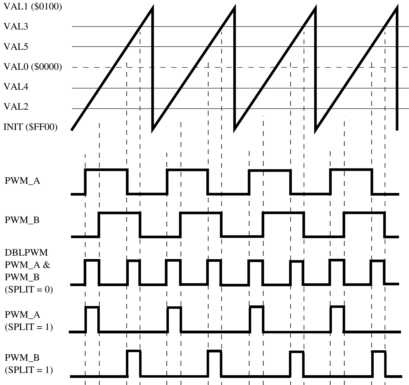
Figure 55-6. Double Switching Output Example
