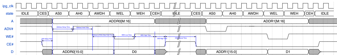
Figure 25-61. SRAM Write in ASYNC mode (ADMUX)
