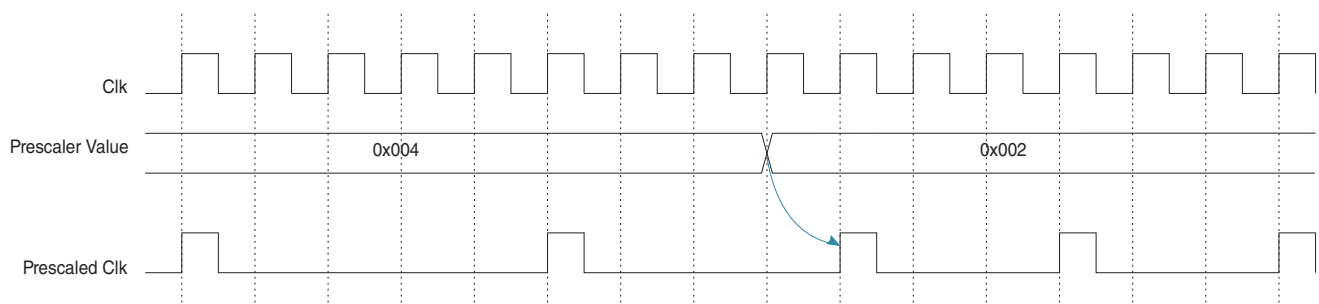
Figure 52-3. Prescaler Value Change Timing Diagram
