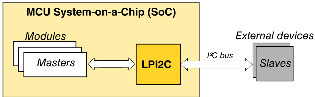
Figure 47-2. LPI2C connects masters in MCU to external slaves on PCB
