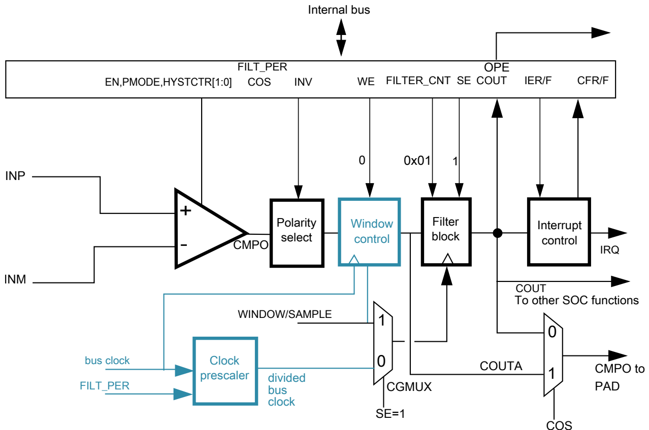
Figure 65-4. Sampled, Non-Filtered (# 3A): sampling point externally driven
