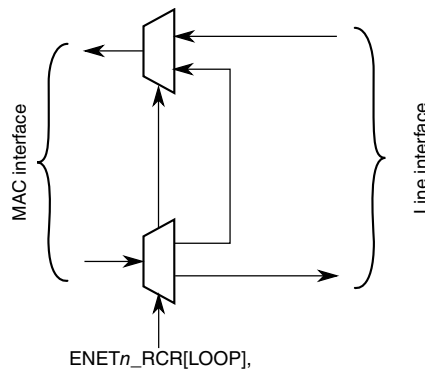
Figure 41-13. Loopback options
