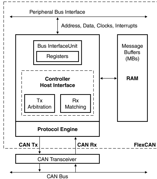
Figure 45-1. FlexCAN block diagram
