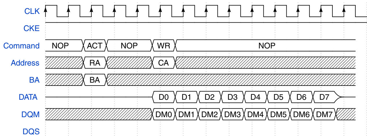
Figure 25-10. IP command - SDRAM WRITE
