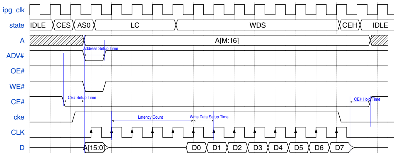
Figure 25-64. SRAM Write in SYNC mode (ADMUX)
