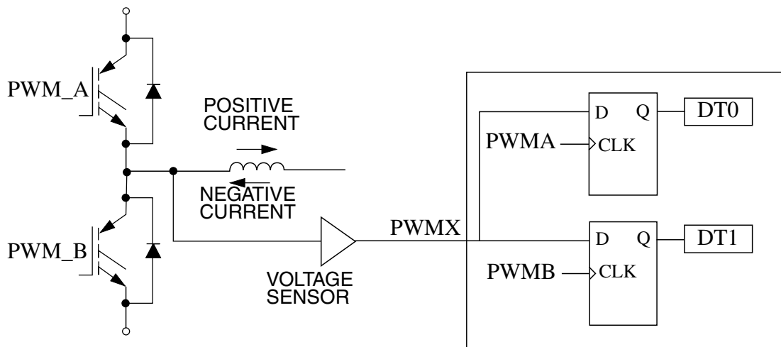
Figure 55-23. Current-status Sense Scheme for Deadtime Correction
