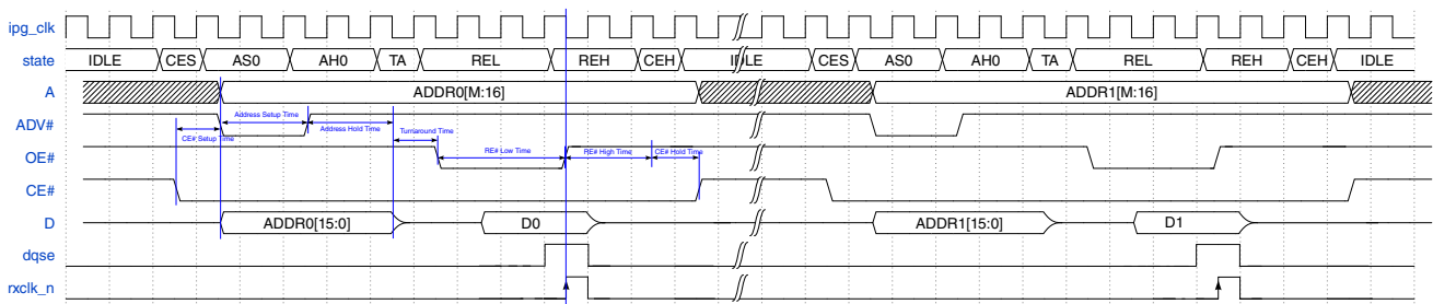
Figure 25-52. Flash Read in ASYNC mode (ADMUX)
