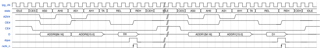
Figure 25-53. Flash Read in ASYNC mode (AADM)
