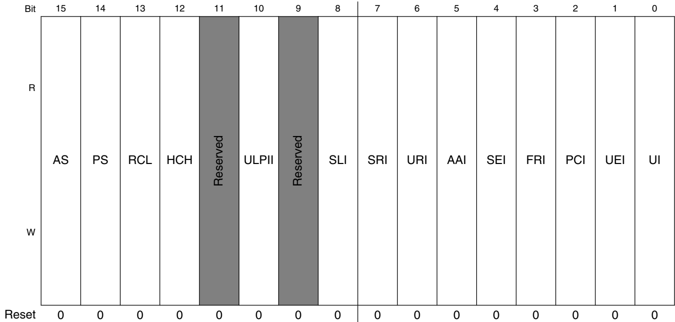
USB_nUSBSTS field descriptions
