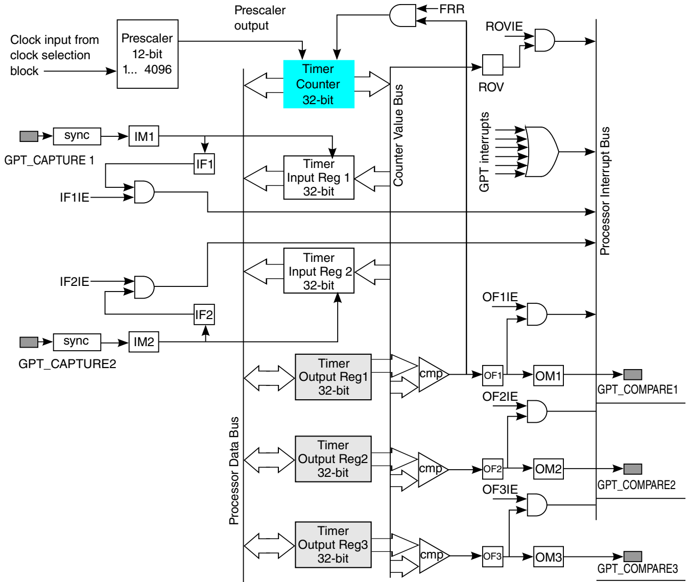
Figure 52-1. GPT Block Diagram
