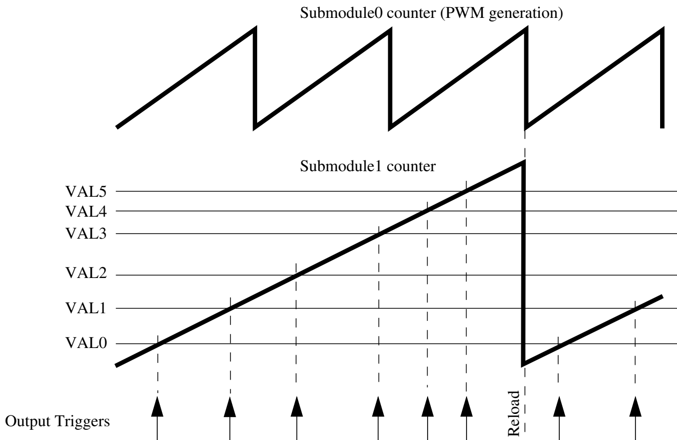
Figure 55-8. Multiple Output Triggers Over Several PWM Cycles
