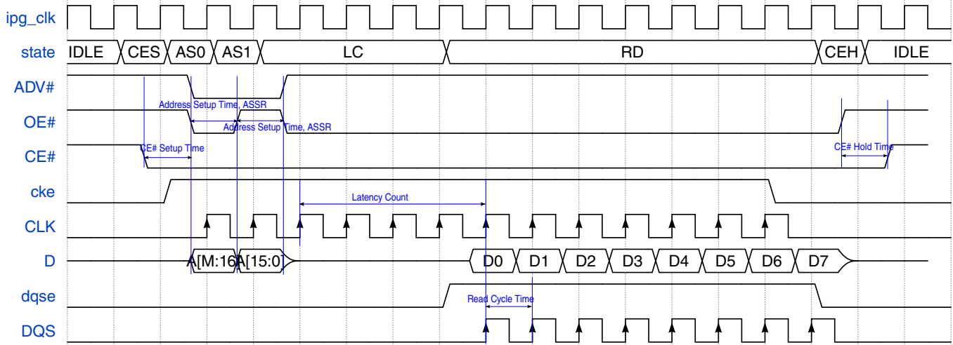
Figure 25-57. Flash Read in SYNC mode (AADM)
