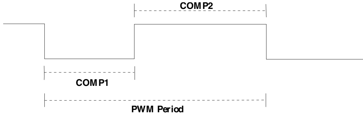
Figure 54-2. Variable PWM Waveform
