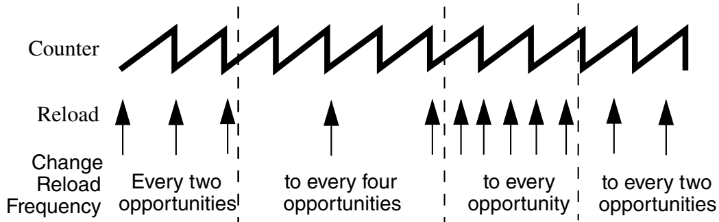
Figure 55-33. Full and Half Cycle Reload Frequency Change
